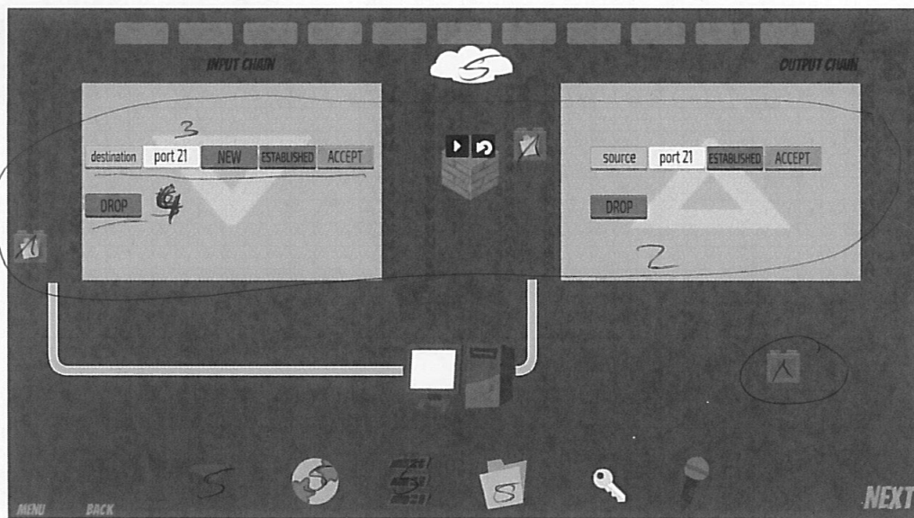
Figure 1: Game Screen
