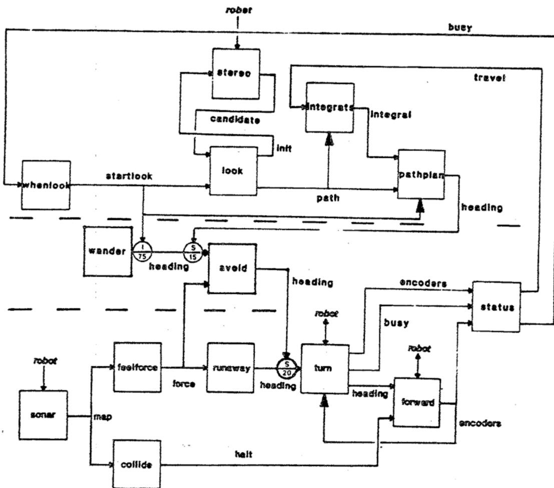
Figure 1. Three layered control system for an exploring robot
