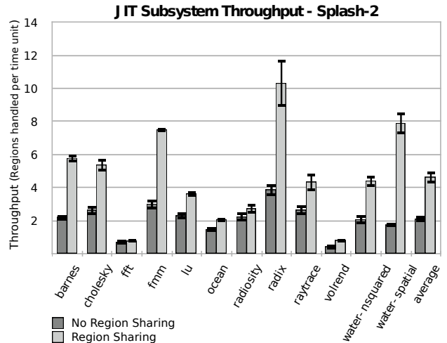
Figure 5. Comparison of JIT subsystem service throughput, with and without region sharing enabled, when executing 128 threads.
