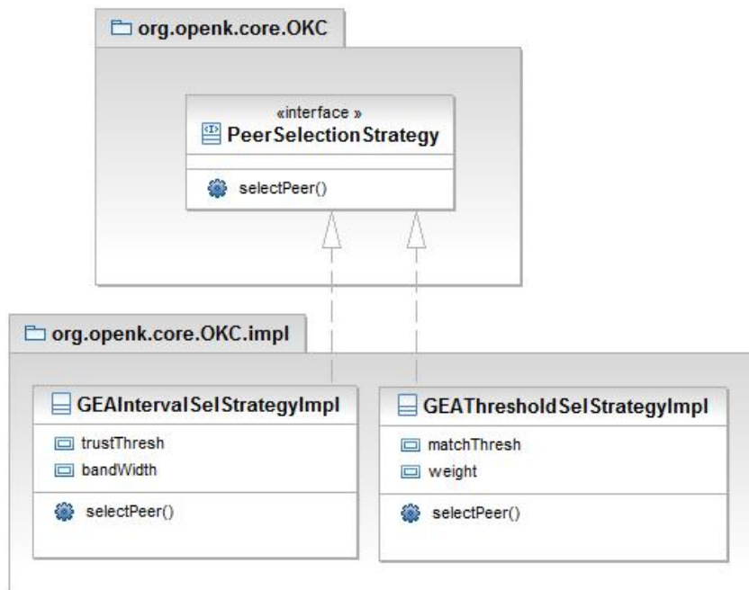
Figure 2: The GEA class diagram.
