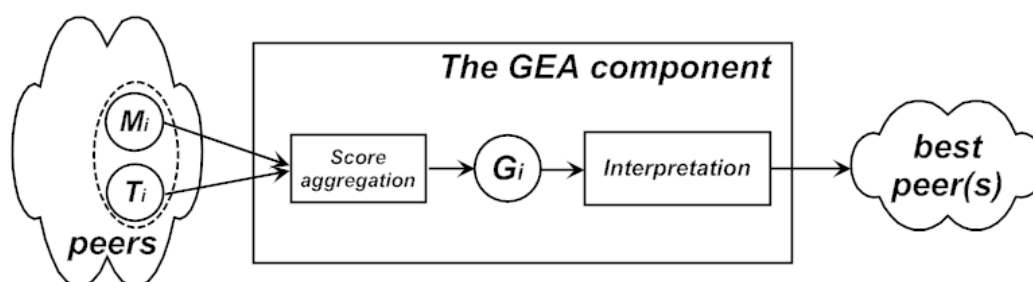
Figure 1: The GEA architecture.
